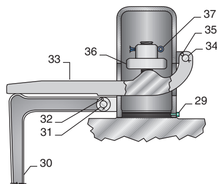
Type C Regular Lifting Gear
