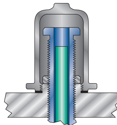
Type A (standard) Threaded Cap
