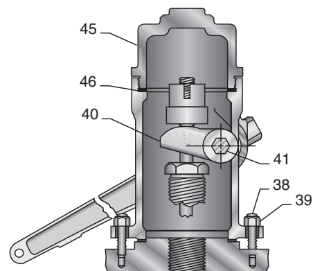
Type D Packed Lifting Gear
